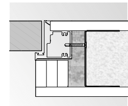
reversed rebate (inward opening)
